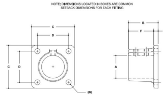
#45CE Square Base Flange SCALE: HALF
