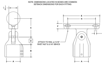
#151 Adjustable Speed Tee SCALE: HALF
