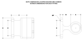
#54-3 Offset Wall Flange (3")
