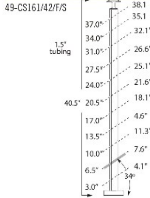
1.5" SQ. Floor Mount Posts
