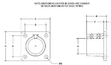
#45CE Square Base Flange
