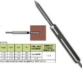
Adjust-A-Body® with Hanger Bolt Tensioner This tensioner screws right into your wooden end post. There is no need for special mounting hardware.
