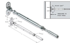
Surface Mount Turnbuckle
