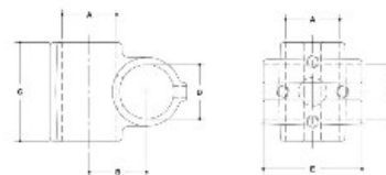
#10-56 Offset Cross
