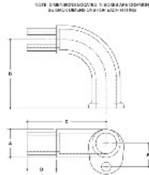
#84L Handrail Return SCALE: 1/4"=1"
