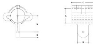
#17SM Modular Male Assembly SCALE: 1/4"=1'
