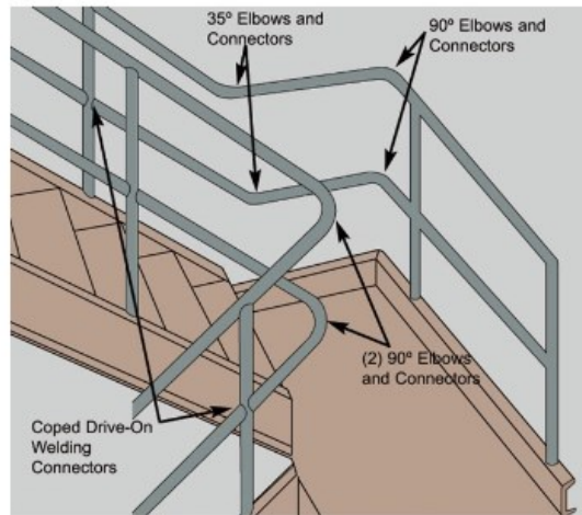
Typical Pipe Stair Railings
