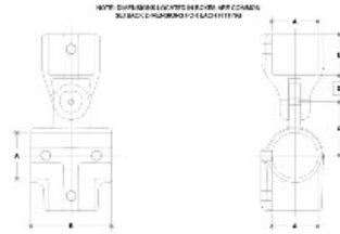
#23 Adjustable Tee or Cross
