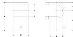
#16 Bolt-On Tee
