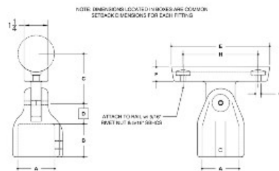
#151 Adjustable Speed Tee
