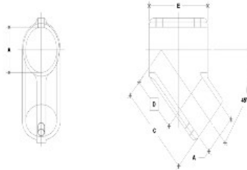
#6 Angle Tee (45°)
