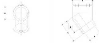
#5AT Angle Tee (55°) DIMENSIONS IN INCHES
