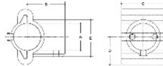
#2S Modular Tee
