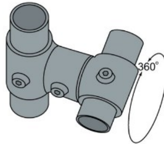
10 and 114 Combination 360° swivel tee for stair railings. This internal swivel connector eliminates the need for specially drilled angle fittings.
