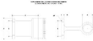
#54-5 Offset Wall Flange (5")
