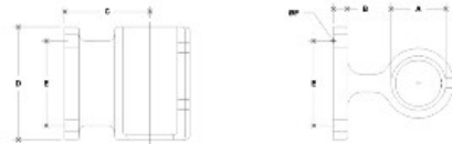
#54-3 Offset Wall Flange (3")
