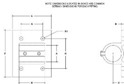
#52 Heavy-Duty Wall Flange SCALE: 1/4" = 1"
