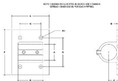
#52 Heavy-Duty Wall Flange
