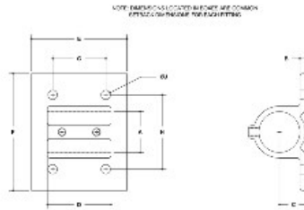
#52 Heavy-Duty Wall Flange
