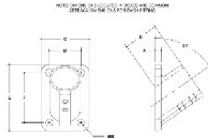
#47AF Angle Base Flange (55°)
