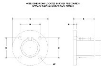
#42 Round Base Flange
