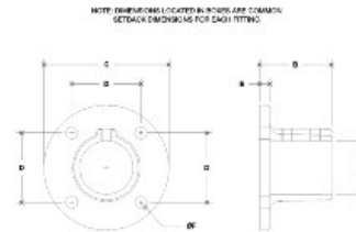
#42 Round Base Flange
