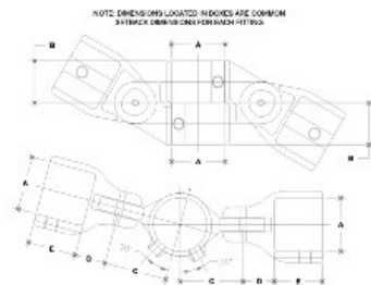
#31 2-Dimensional Adjustable Cross
