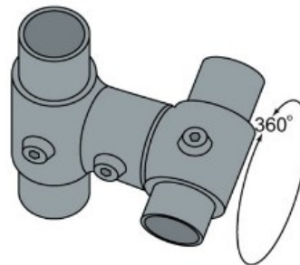
10 and 114 Combination 360° swivel tee for stair railings. This internal swivel connector eliminates the need for specially drilled angle fittings.
