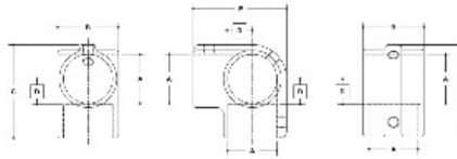
100% ANODIZED ALUMINUM FITTING APPROX. DIMENSIONS FOR REFERENCE
