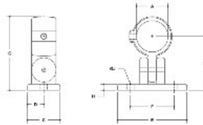
#56 Adjustable Wall Bracket
