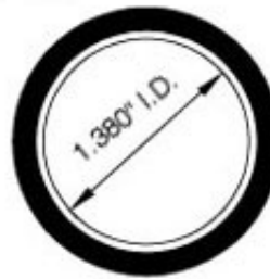
1-1/4" IPS 1.660", 42mm O.D. Schedule 40: 1.380" I.D., 0.140" Wall
